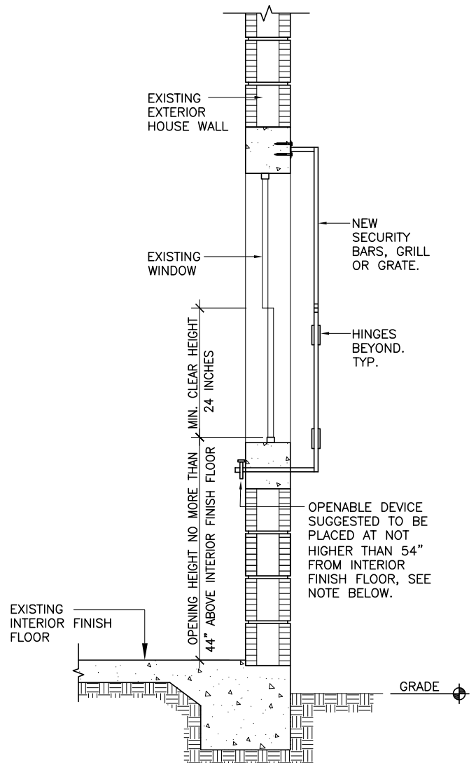
SECTION
