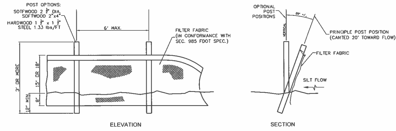
TYPE III SILT FENCE (TYP.)
