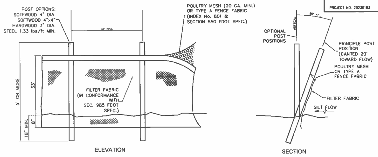
TYPE IV SILT FENCE (TYP.)
